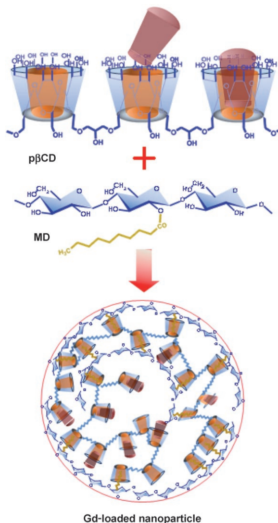
Figure 1. Formation of Gd III -loaded nanoparticles through a supramolecular three-component assembly: Gd III chelate/p \beta CD/MD. The alkyl chains functionalizing dextran are in yellow, the Gd III chelate is in violet.
