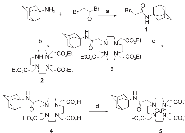
Scheme 1. Synthesis of the Gd III chelate: a) CH 2 Cl 2 , Na 2 CO 3 , RT; b) CH 3 CN, K 2 CO 3 , RT; c) EtOH/H 2 O, AG1-X4 resin (OH Form), RT; d) GdCl 3 , H 2 O, RT.
